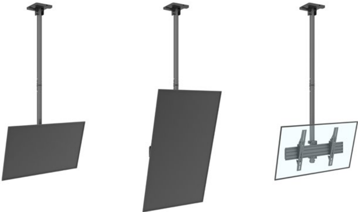
Ceiling Signage stand – Single screen. Extendable length, heavy duty steel construct, tilting brackets for optimised viewing options, and Vesa compatible mount.
