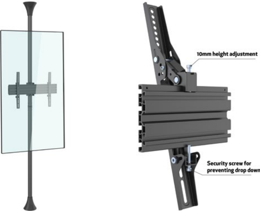
Floor to Ceiling Signage stand. Extendable to 3m, small footprint, single or multi screen, adjustable screen height, heavy duty steel construct, Vesa compatible mount, microphone option, and storage.
